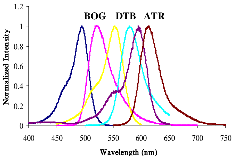
Figure 2. Normalized excitation and emission spectra of BOG, DTB and ATR.
