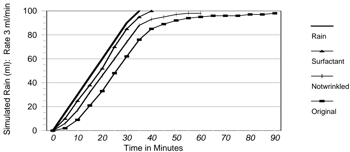
Figure 2 - CS 705 Overflow Tube Shape Analysis: Recuperation Time Comparison
