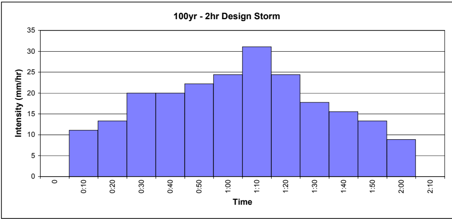
Figure 2.7 - Rainfall Hyetographs 1 in 100-year Return Period
