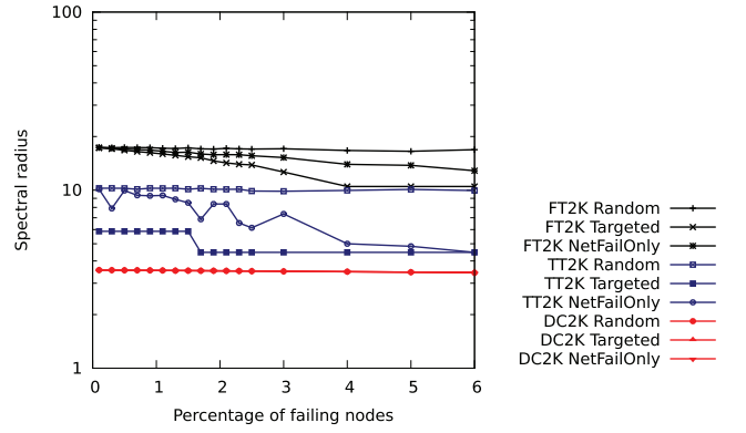
Fig. 8. Spectral radius analysis of the 2K networks.
