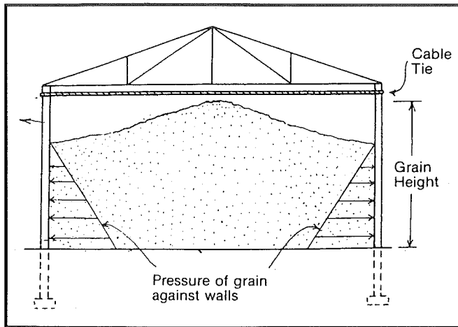
Figure 1. Use a cable to tie post tops together or walls may pull apart from roof. (NRAES-1 Pole and Post Building Construction, 1977.)
