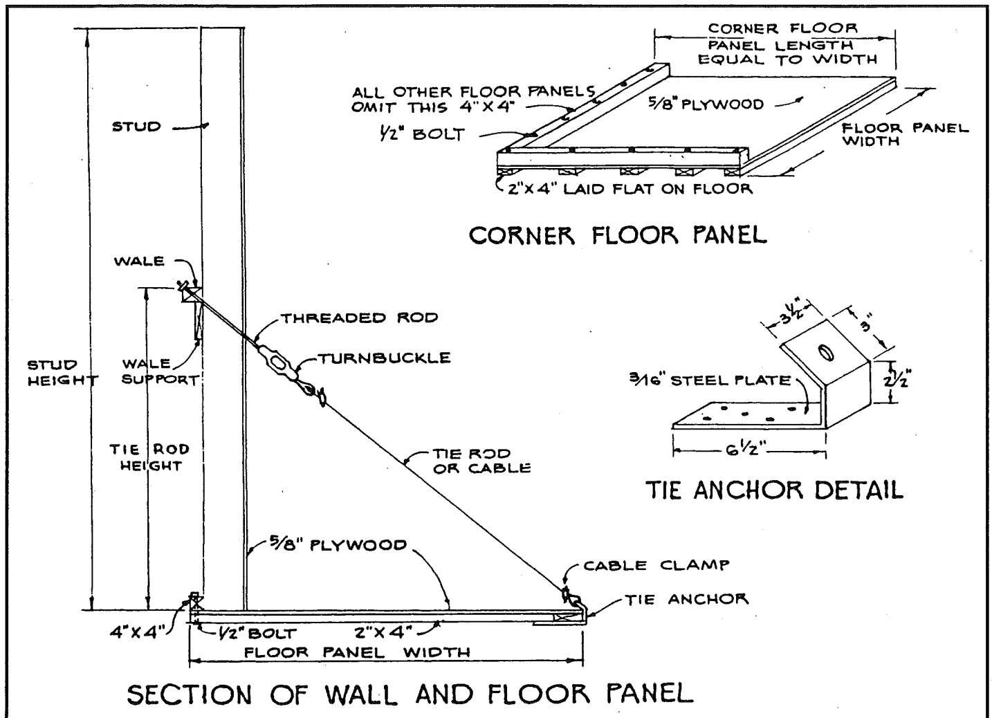
Figure 5. Details of self-supporting portable wall.
