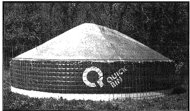
Figure 7. Sidewalls on this type of storage are reinforced with wire mesh and used to support walls 4 feet to 6 feet high. Covers can be reinforced plastic sheeting. Bins are filled with augers. (Suppliers of this type include: B & W Mfg Co., Columbus, NE 402/564-3032 and Thompsons, Melita, Manitoba 204/522-3241.)
