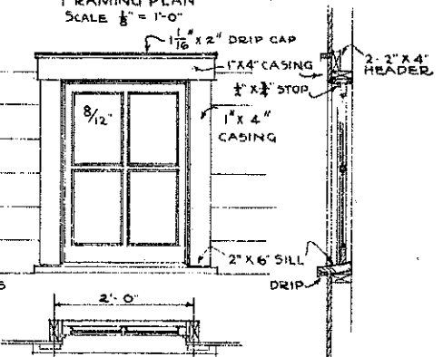
DETAIL OF WINDOW SCALE \frac{1}{2}'' = 1'-0''
