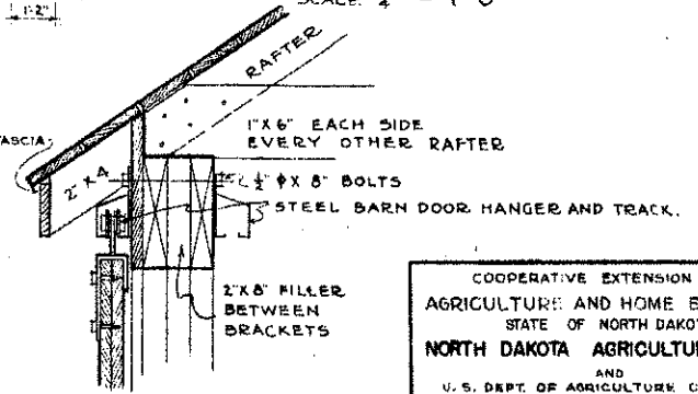
DETAIL OF LINTEL OVER ROLLING DOORS SCALE \frac{1}{2}'' = 1'-0''
