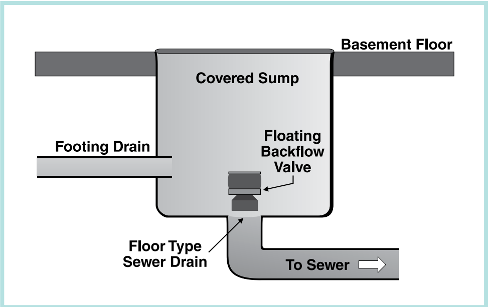
Figure 20. Footing drain.
