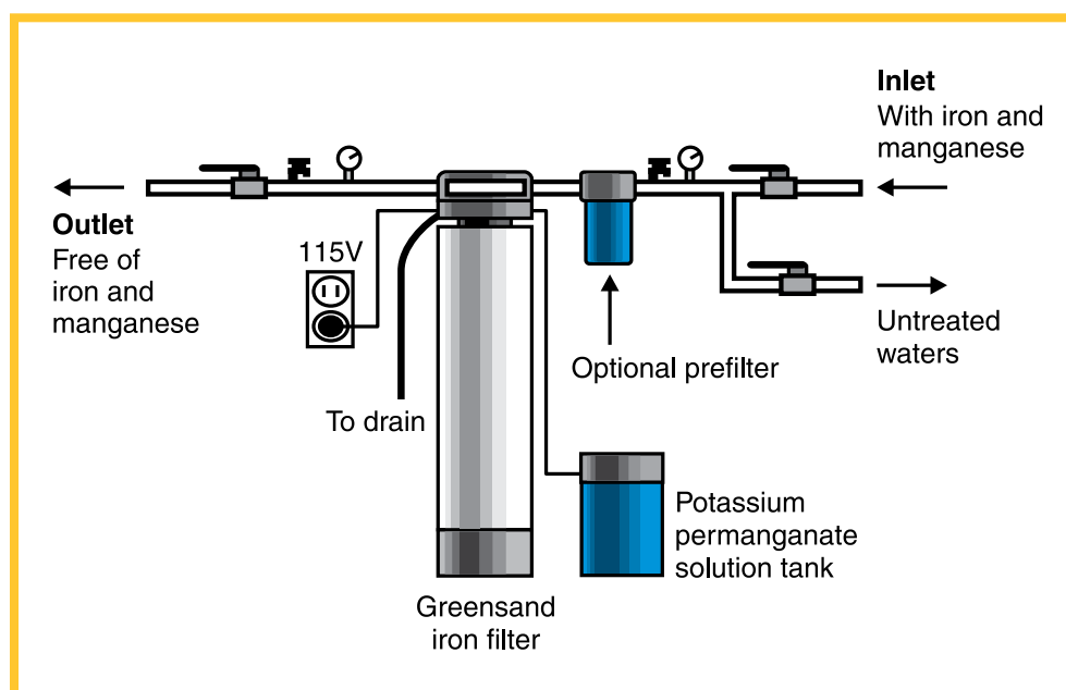
Figure 1. Greensand filter.
