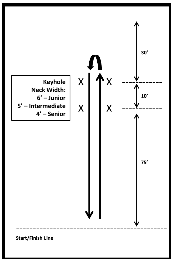
Figure 20. Keyhole Pattern
