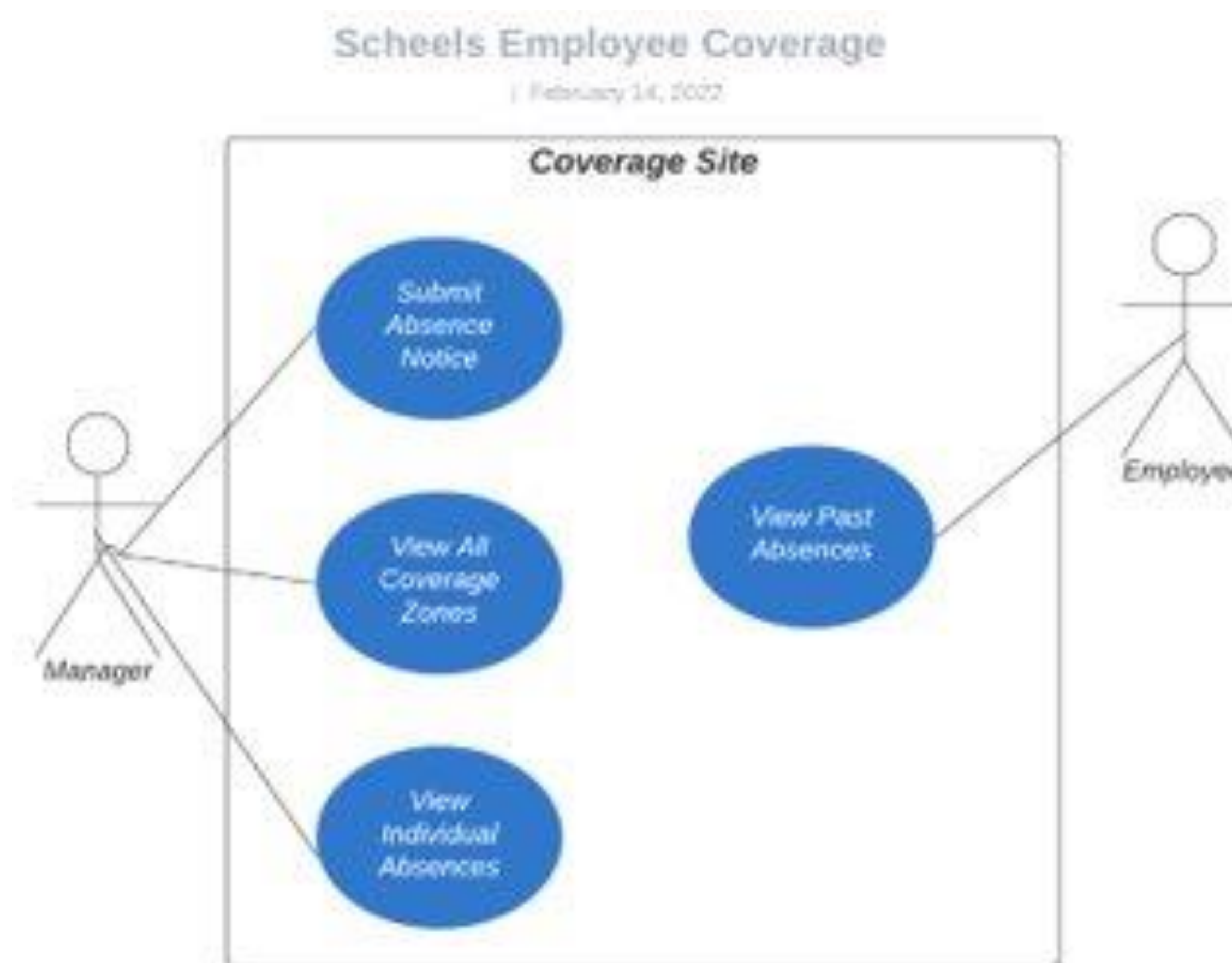
UML Diagram
