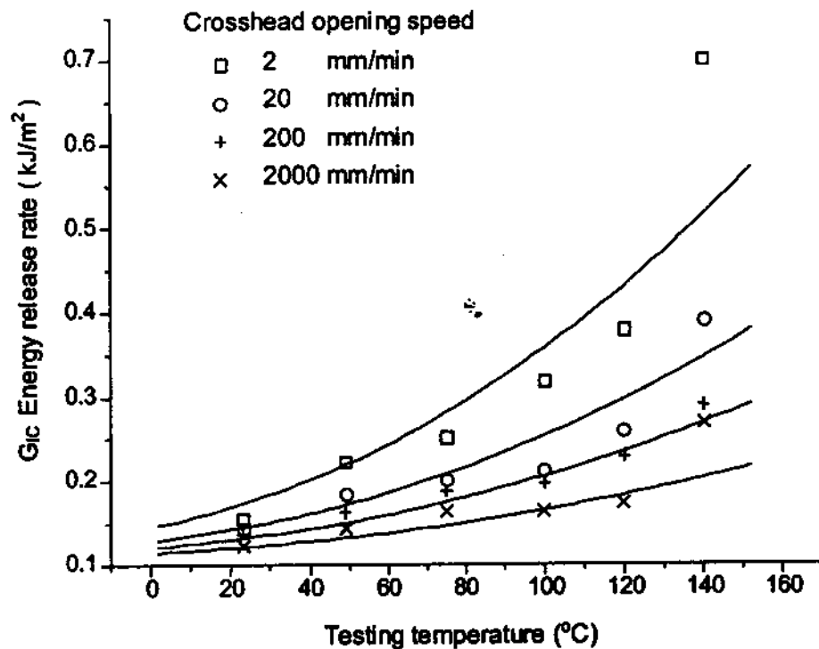
Figure 1. Variation of G_{IC} with loading rate and temperature (Scatters--experimental results, solid lines--calculated by (6))
