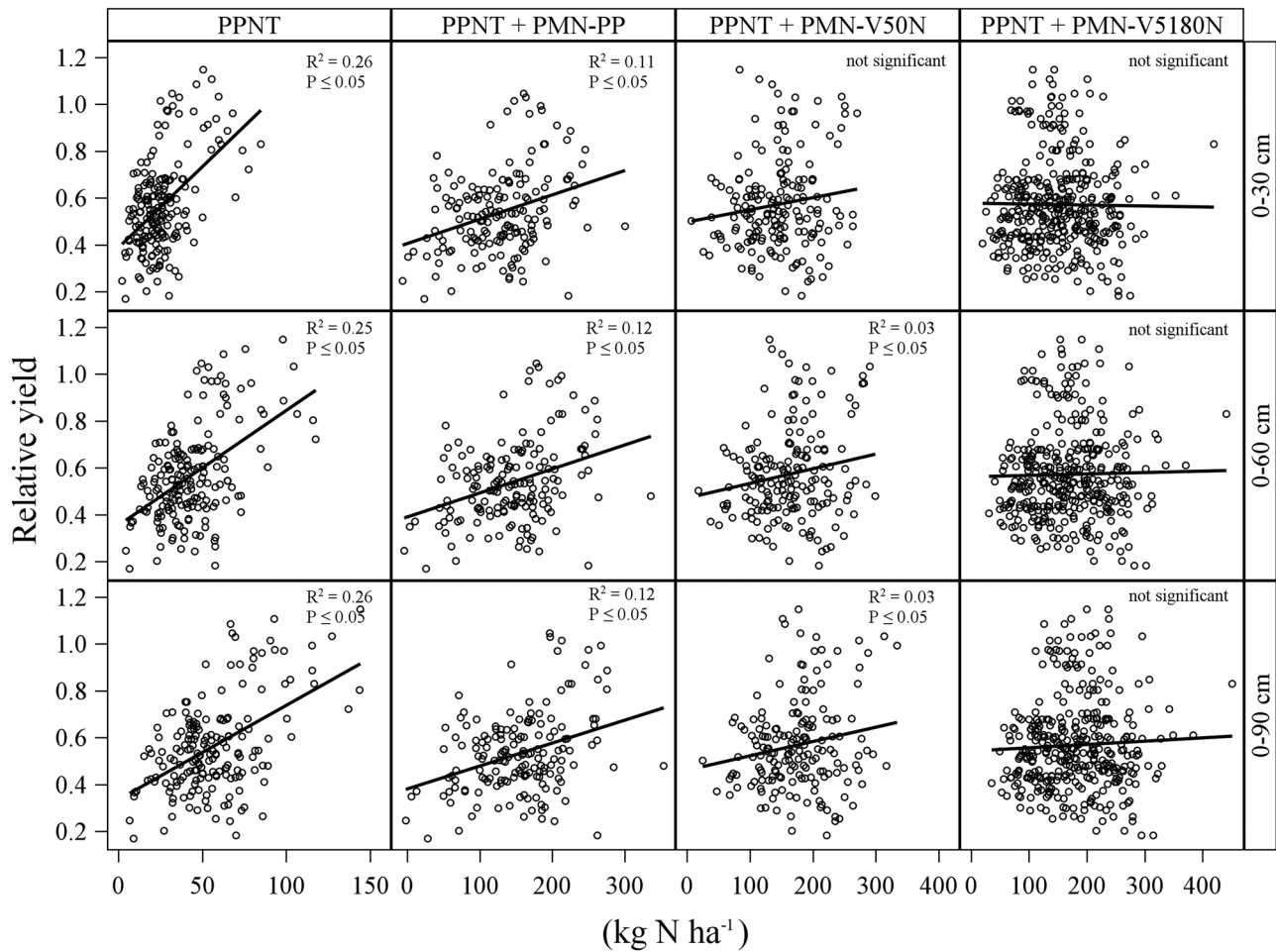
FIGURE 1 In 0 kg N ha -1 plots across 49 site-years, relationship between relative corn yield and soil NO 3 -N content before planting and fertilization at three depths (PPNT) and PPNT combined with anaerobic potentially mineralizable N (PMN) from three sampling methodologies (soil sampled before planting and N fertilization [PPNT + PMN-PP], soil sampled at the V5 corn development stage where 0 [PPNT + PMN-V50N] or 180 kg N ha -1 [PPNT + PMN-V5180N] was applied at planting)
