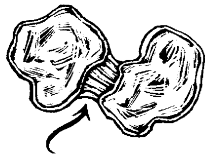
Capillary water is held in the pore space against the force of gravity.
