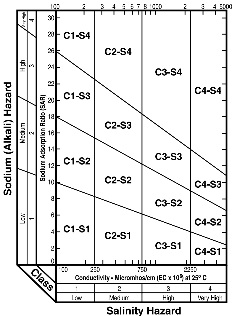
Figure 5. Diagram showing the classification of irrigation water. (From Agriculture Handbook No. 60, USDA Salinity Laboratory in Riverside, Calif.)
