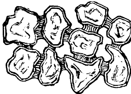
Field capacity. The capillary pores are full and the remaining pore space is filled with air.
