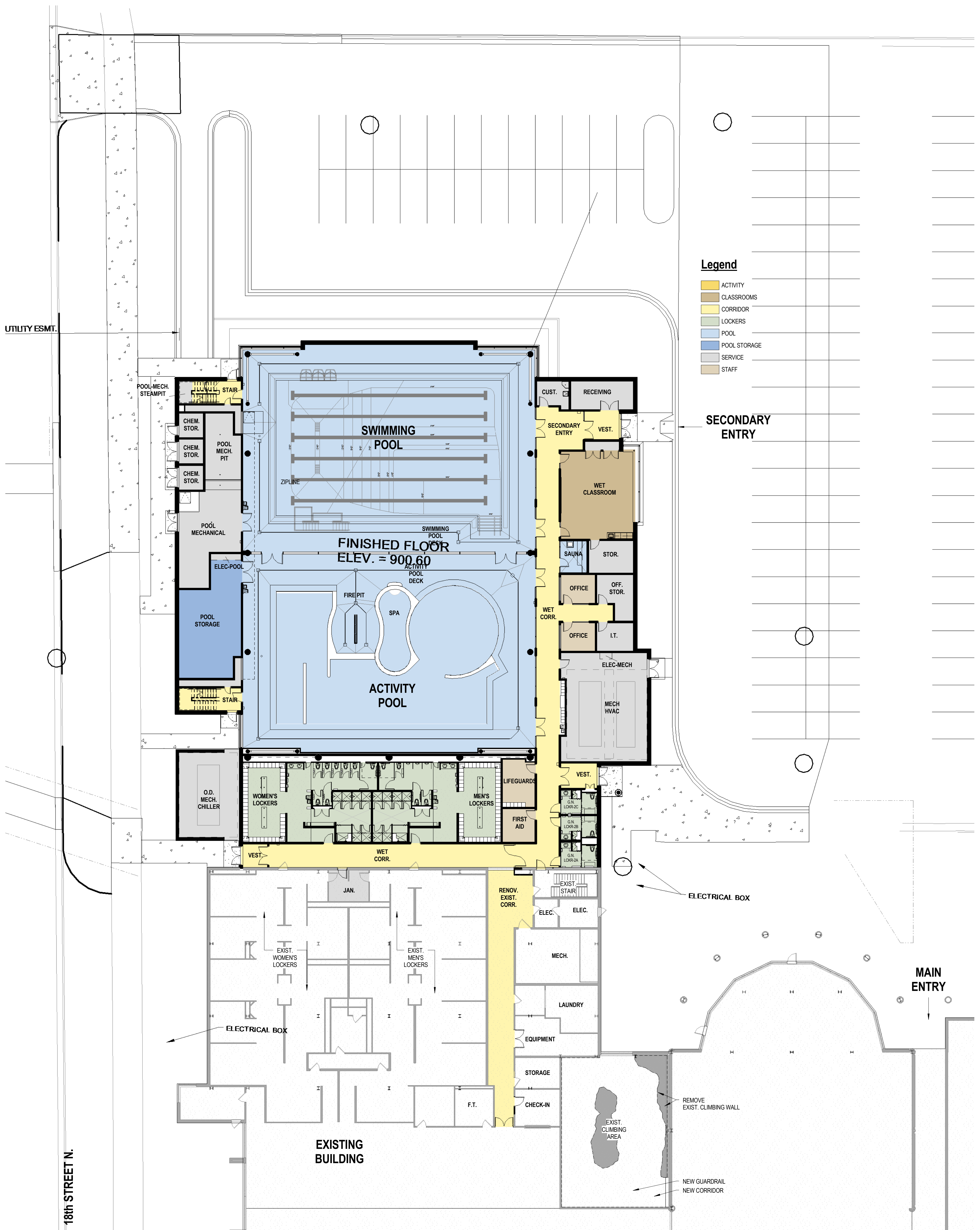
1 1st FLOOR PLAN - PRESENTATION 1/16" = 1'-0"
