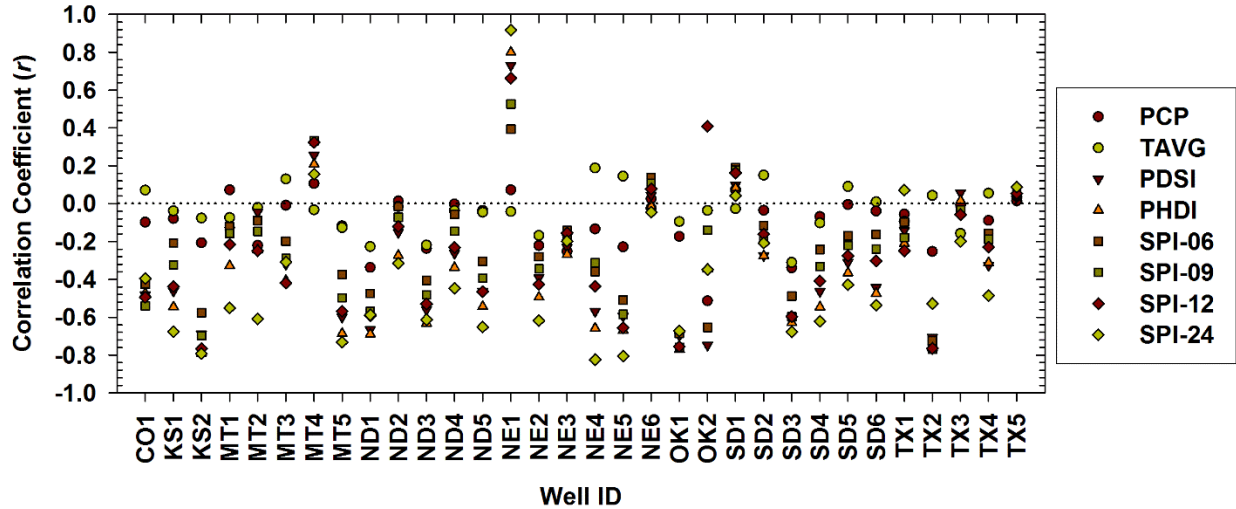
Figure 3.2: The Pearson correlation coefficient, r , between groundwater level ( b ) and drought indices.
