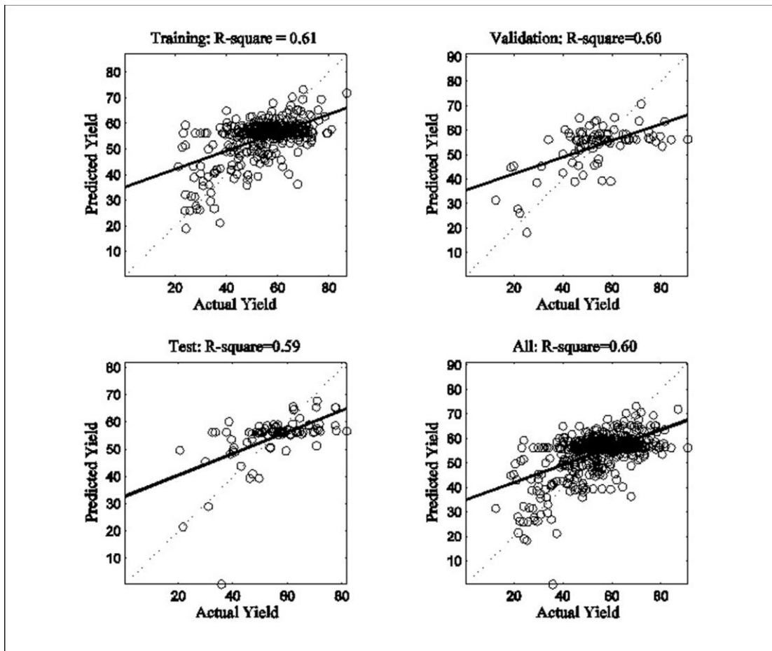
Figure 4.4: The relationship between actual and predicted yield of barley using ANN.
