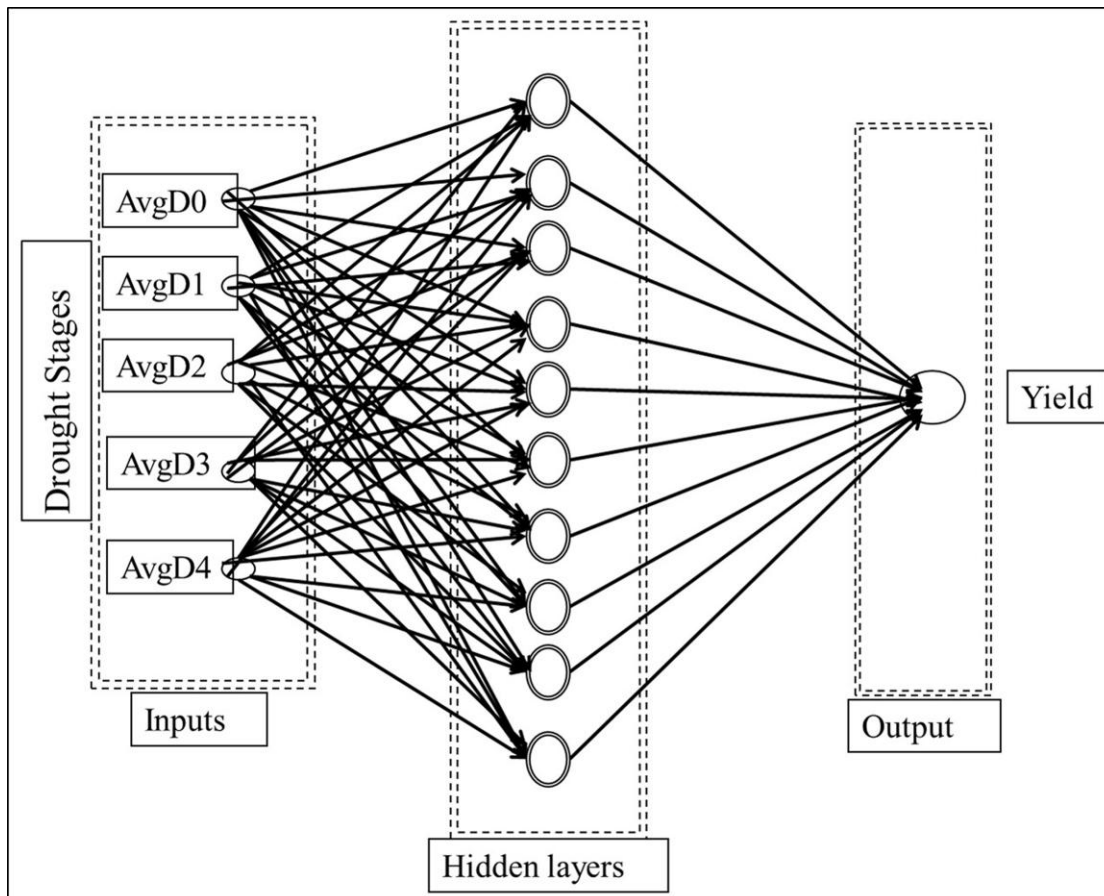
Figure 4.3: ANN Scheme for the study problem.
