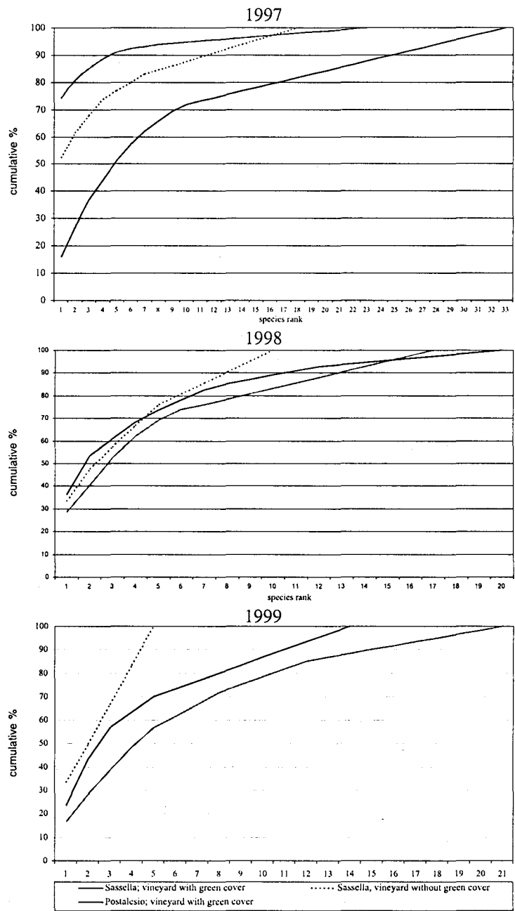
Fig. 1 - Cumulative curves of Heteroptera in the three vineyards.
