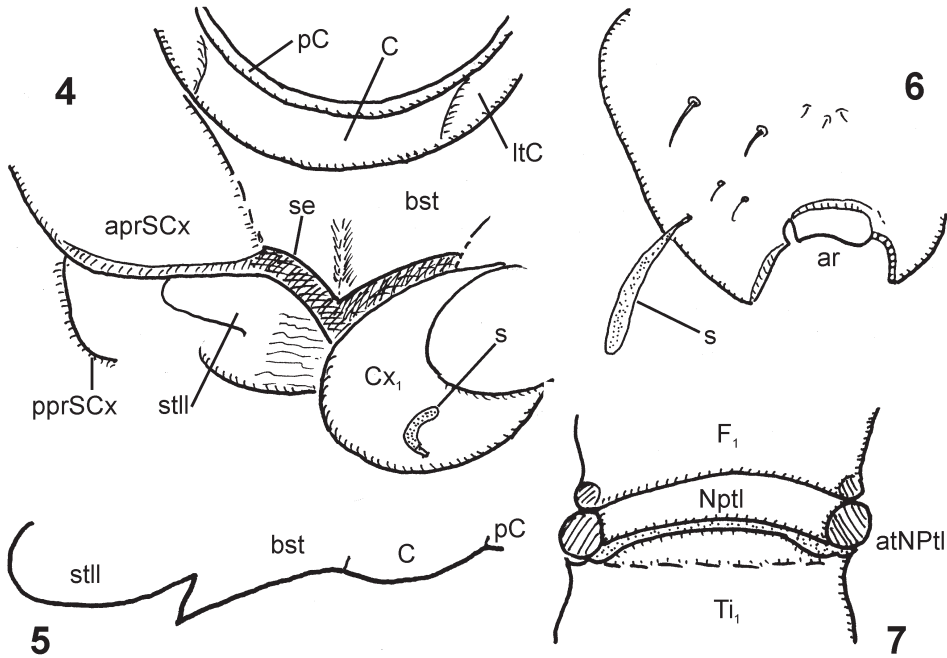
Figs. 4-7. Systelloderes loebli sp. nov., holotype, female. 4 – prosternum and associated structures, posteroventral view, diagrammatic; 5 – prosternum, sagittal section, diagrammatic; 6 – right fore coxa with a scale; anterior (mesal) view; diagrammatic; 7 – neopatella; lateral (dorsal) view on bent ‘knee’ of left fore leg; diagrammatic. Lettering: aprSCx – anterior prosupracoxale; ar – coxo-trochanteral articulation; atNptl – articular tubercles of neopatella; bst – probasisternum; C – collum; Cx 1 – fore coxa; F 1 – fore femur and its articular processes; ltC – lateral tubercle of collum; Nptl – central part of neopatella; pC – precollum; pprSCx – (edge of) posterior prosupracoxale; s – coxal scale; se – stridulatory edge of basisternum; stll – prosternellum; Ti 1 – fore tibia with a subdivided apex.
