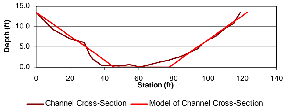
Figure 53. Comparison of the cross-sectional model to the layout of the cross-section for Big Coulee near Churches Ferry, ND.
