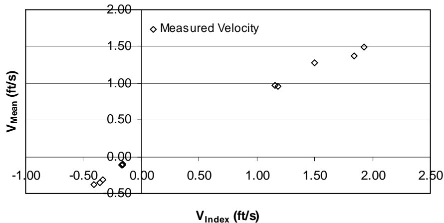
Figure 48. Index-mean velocity relation for Channel A near Penn, ND.
